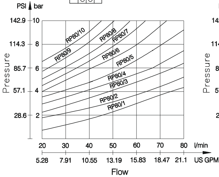
Pressure drop
